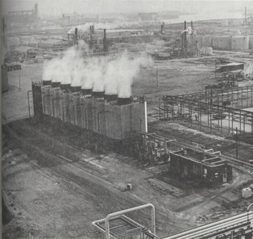
Another view from atop the cat. cracker taken in 1946 (above) and 1974 (below). In the '46 view, you find the CWT #7 and the control building for the recently completed cat. cracker. Today, your view from the same spot would show (from l-r) the naphtha extraction unit, the MEK dewaxing and deoiling unit, the desulfurizer, and (in the background) the Greer Wax Molding Plant.
